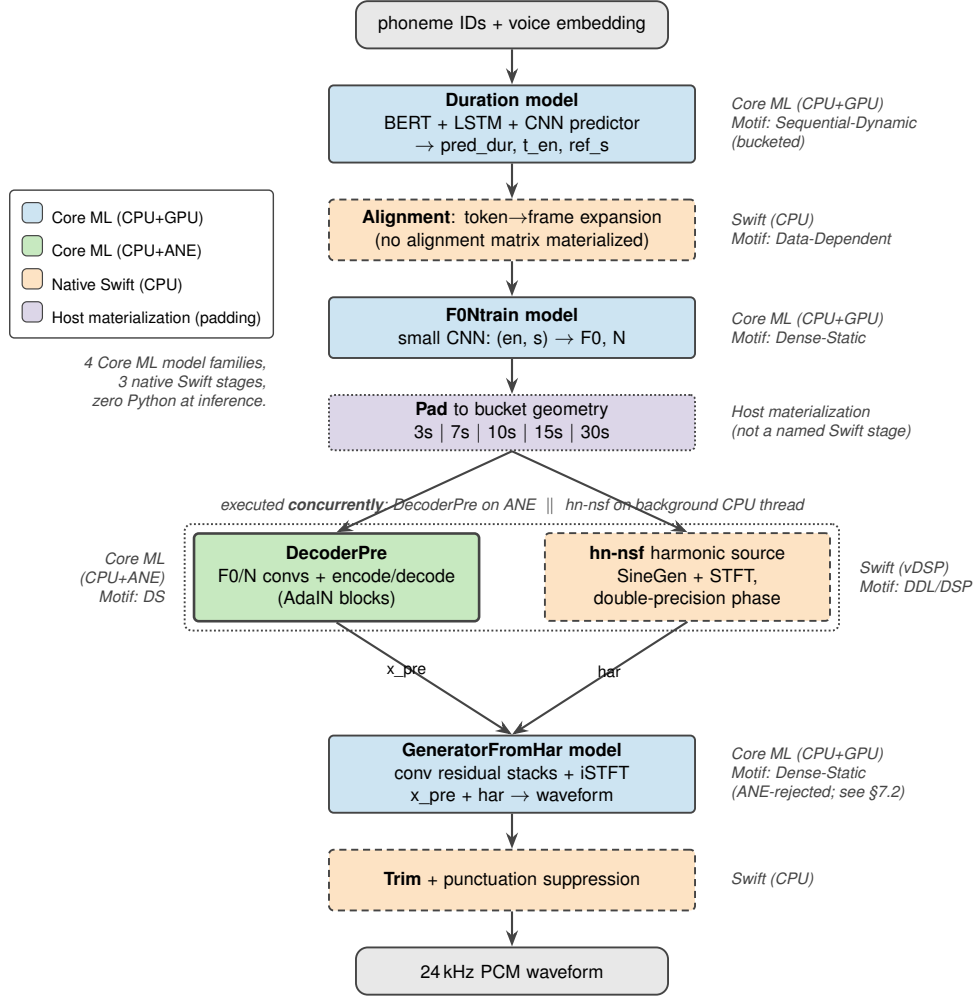
Figure 1: The decomposed Kokoro-82M pipeline: four Core ML model families and three native Swift stages, zero Python at inference time. Each stage is classified by computational motif and placed on the SoC engine that measurement selects (color = placement); only DecoderPre is admitted to the ANE, while the geometry-rejected GeneratorFromHar and the sequential Duration model run Core ML on CPU+GPU. The decomposition also exposes cross-unit parallelism a monolithic graph cannot express: DecoderPre (ANE) and the hn-nsf harmonic source (background CPU thread) execute concurrently.
