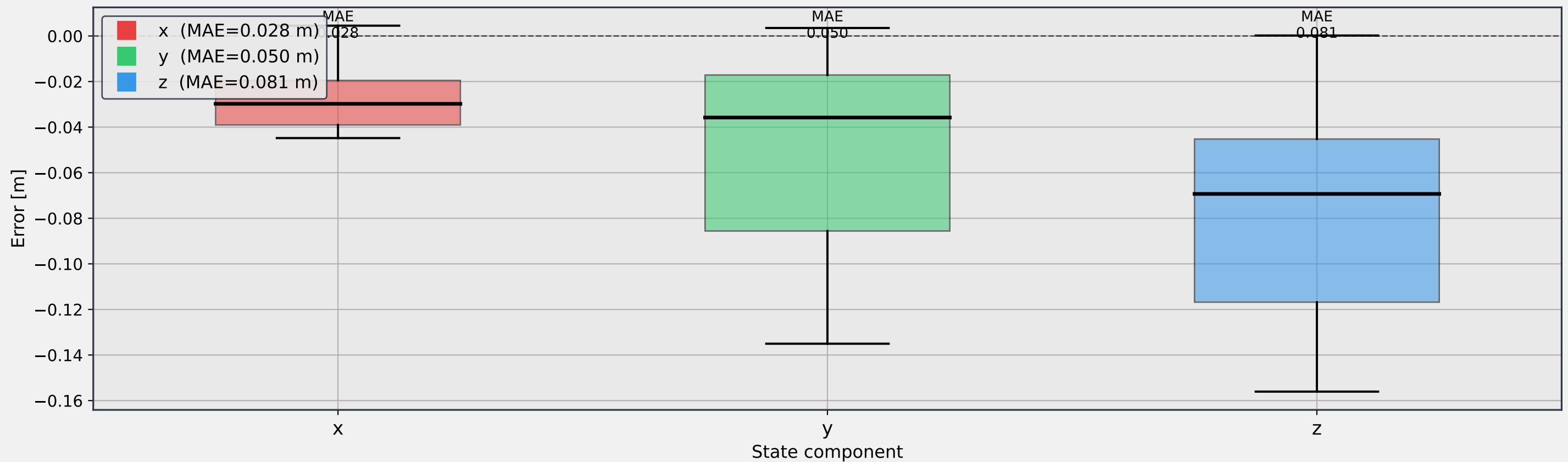
Position error (actual – commanded) - Error Distribution
