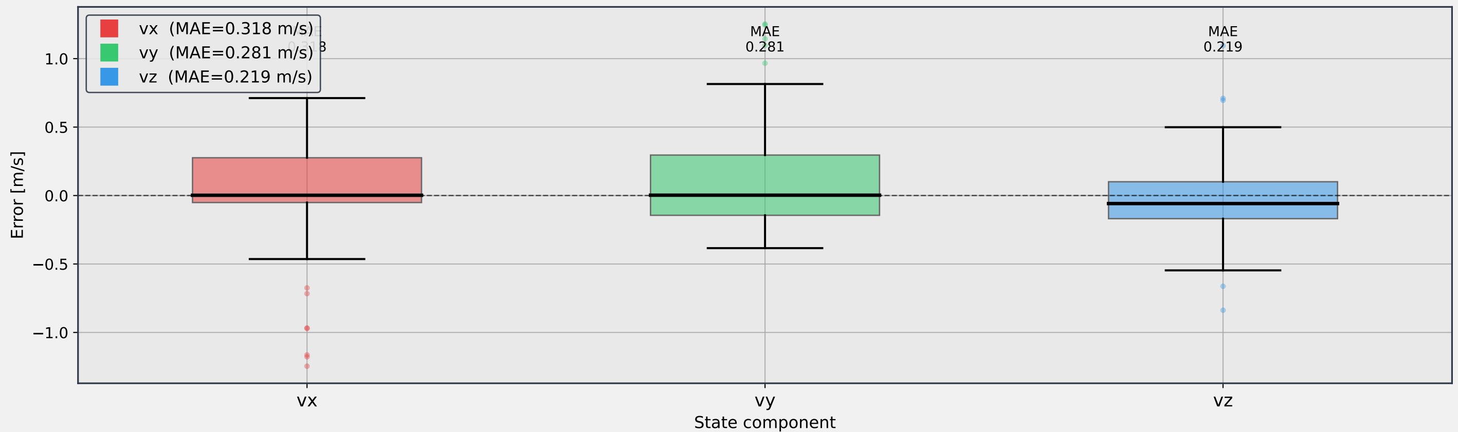
Velocity error (actual – commanded) - Error Distribution
