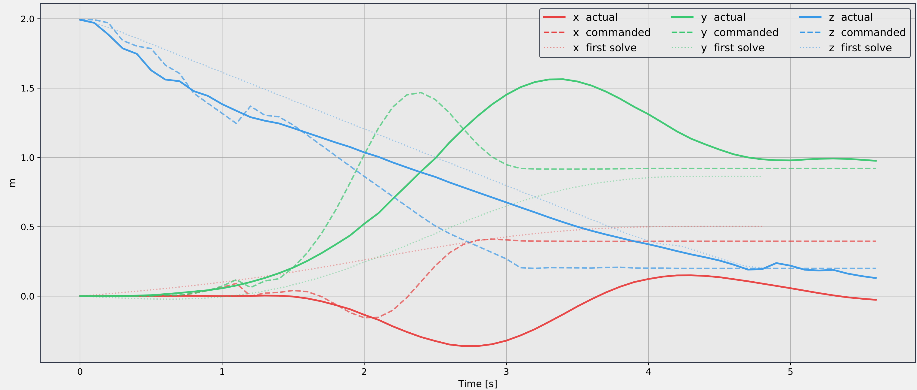
Absolute Position [x, y, z]
