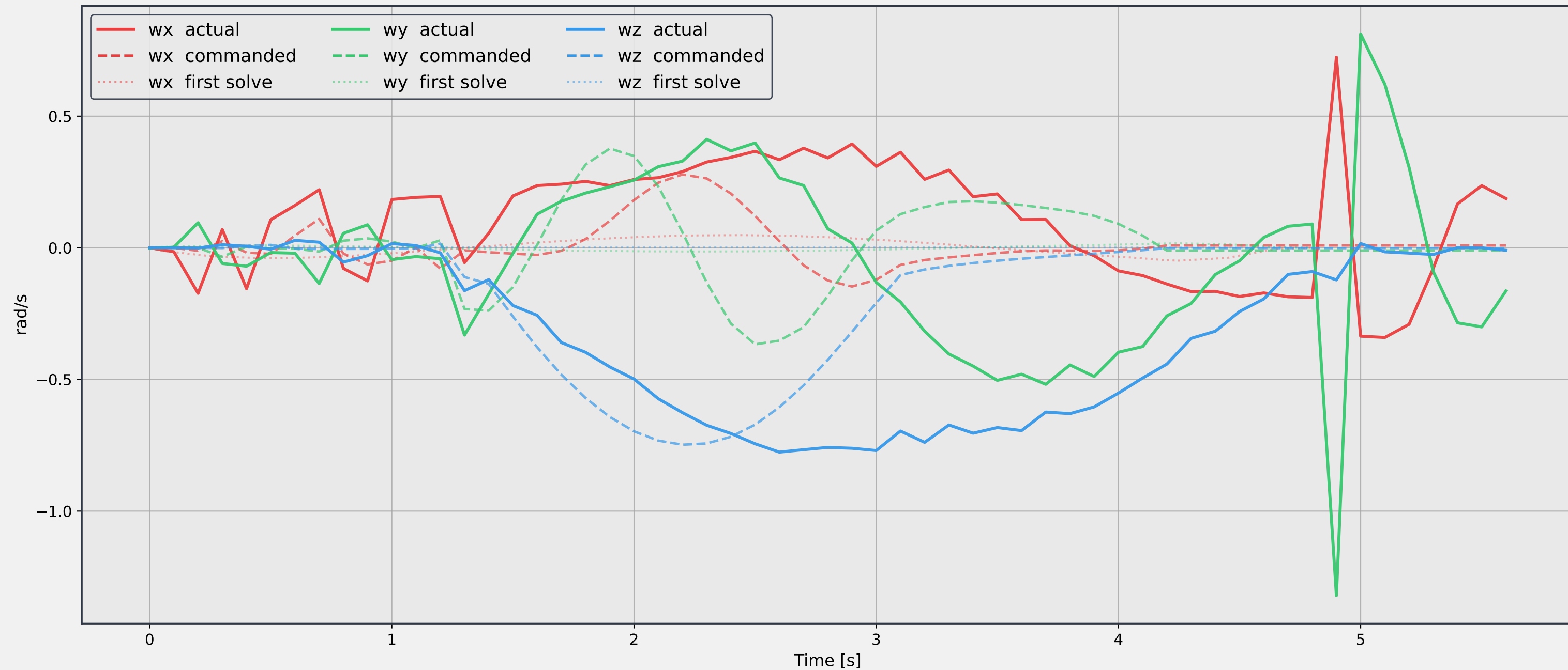
Angular velocity [wx, wy, wz]
