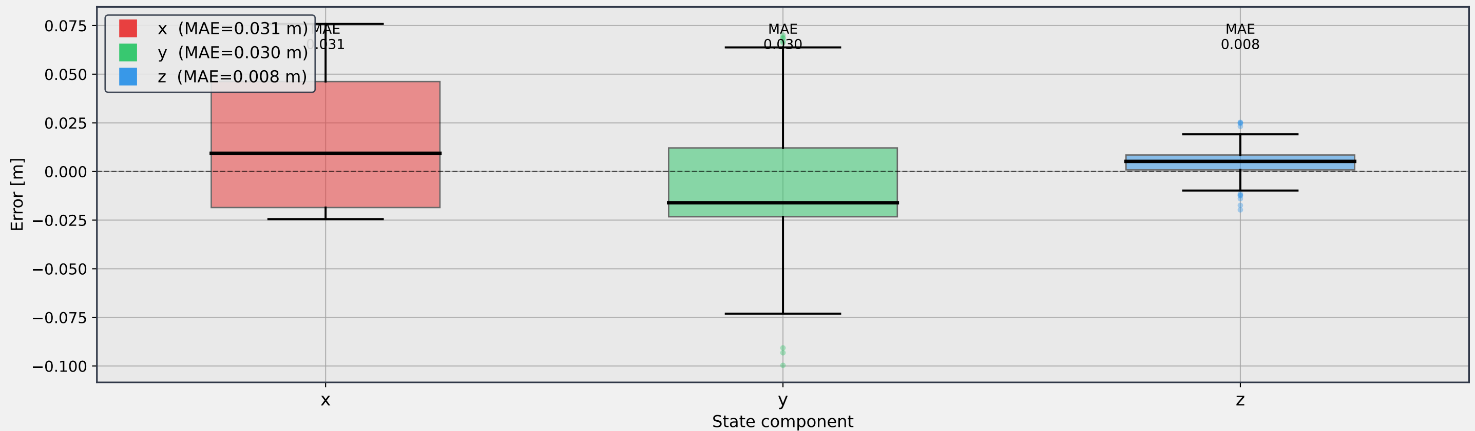
Position error (actual – published command) - Error Distribution
