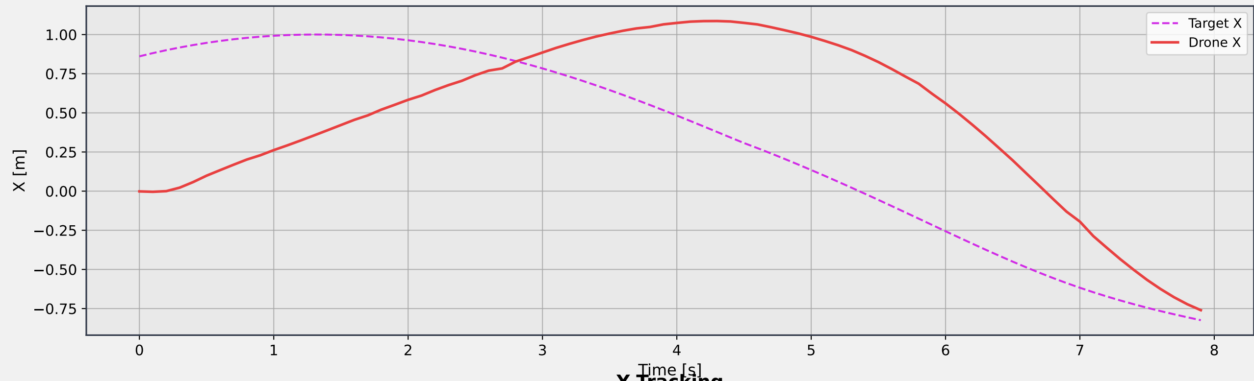
X Tracking
