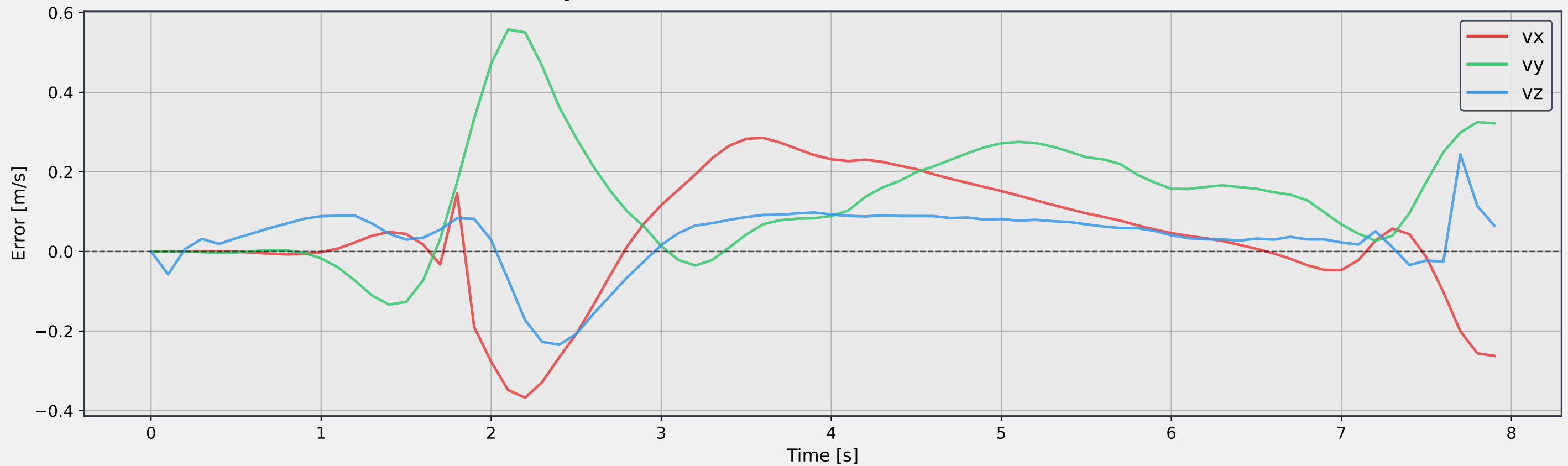
Velocity error (actual – commanded) - Error Time Series
