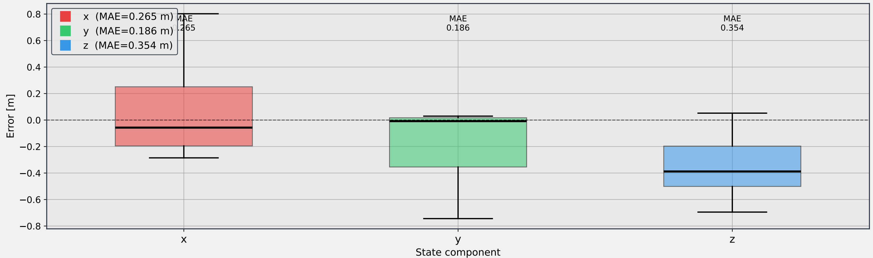
Position error (actual – published command) - Error Distribution
