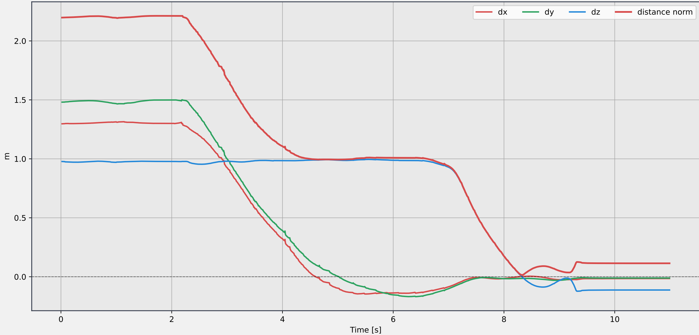
Drone - target world error
