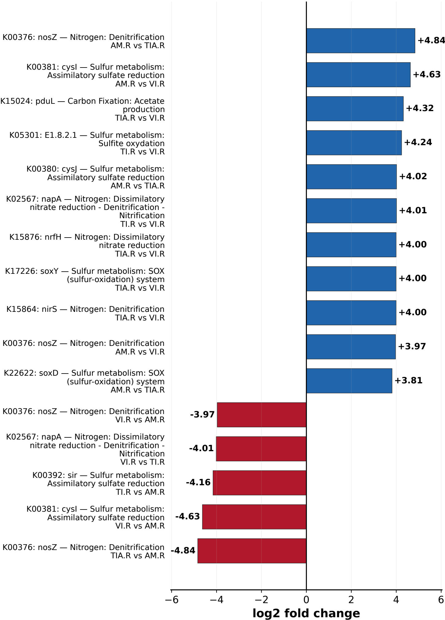
B Rainy-season contrasts
