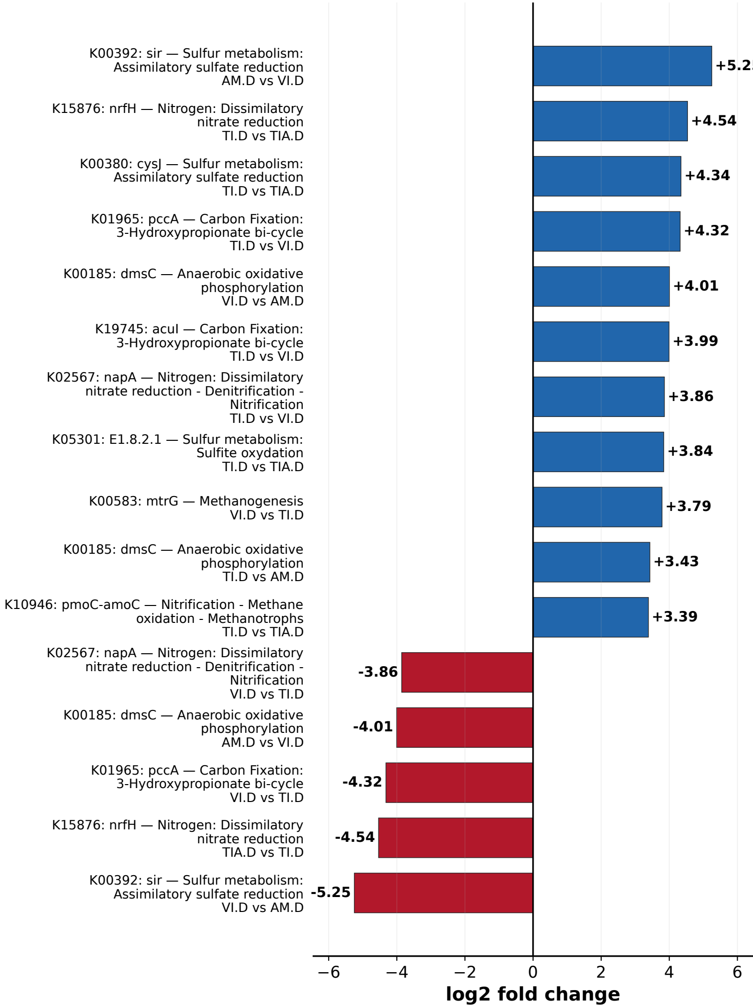
A Dry-season contrasts
