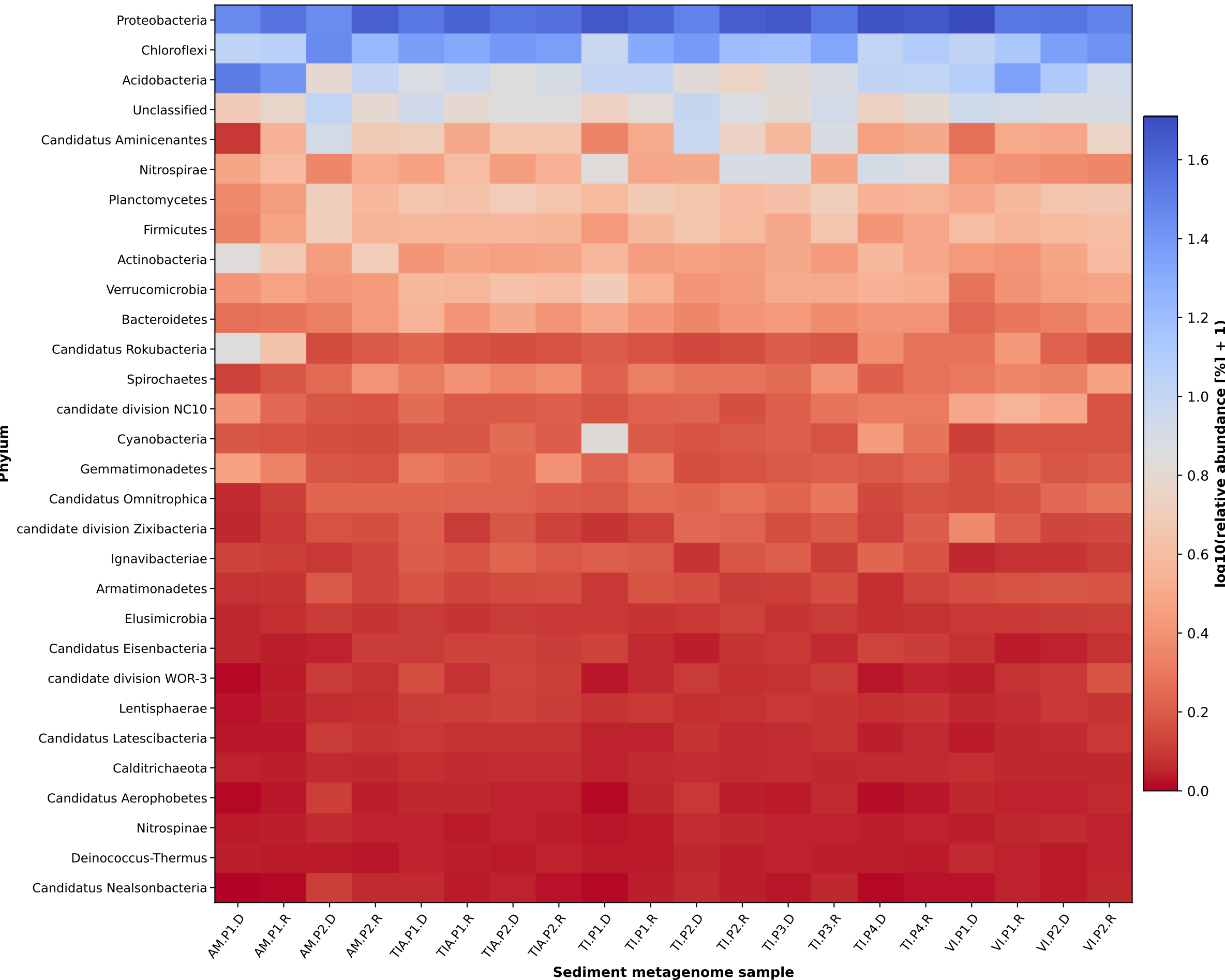
Bacteria — Phylum — relative-abundance heatmap [log10(x + 1)]
