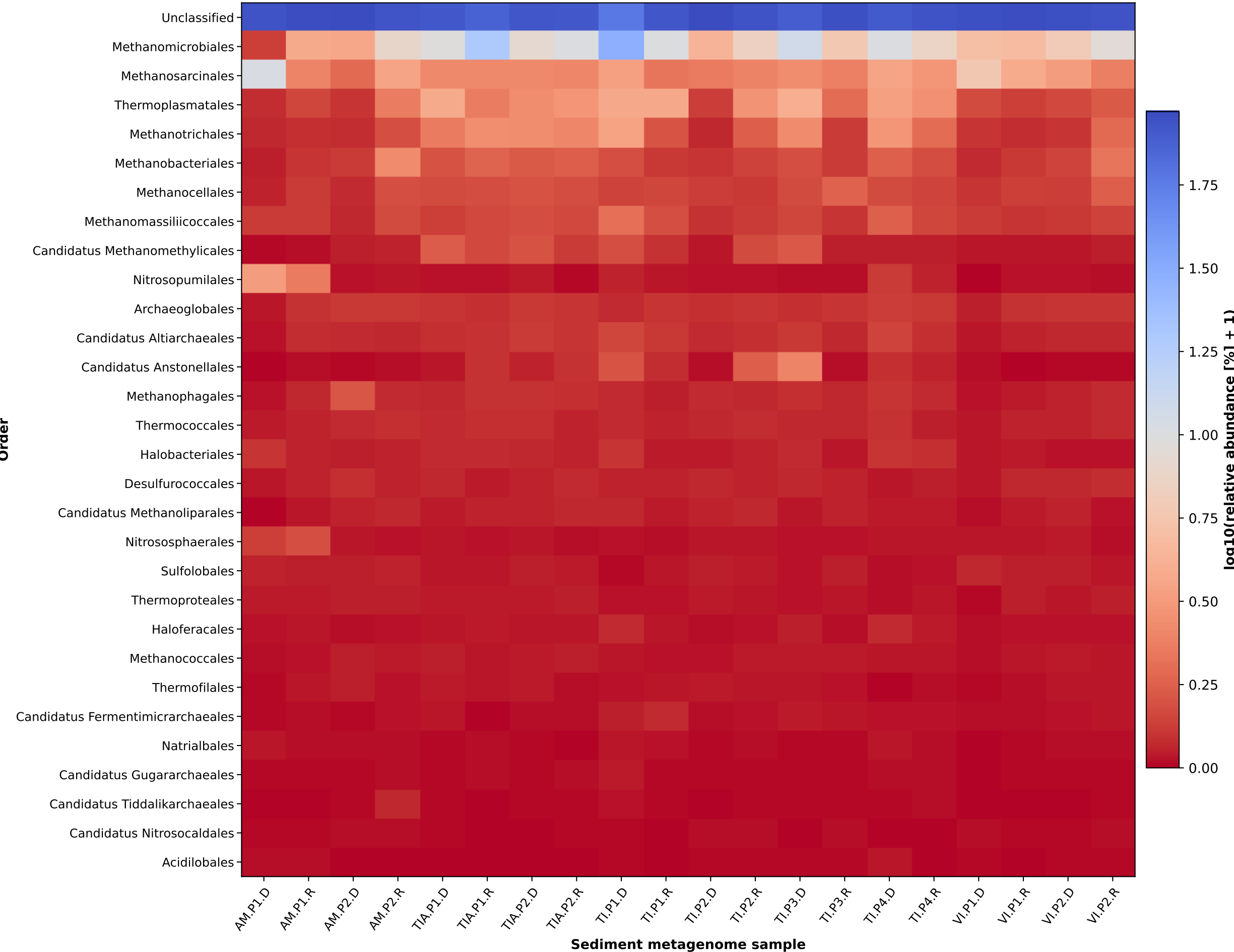
Archaea — Order — relative-abundance heatmap [log10(x + 1)]
