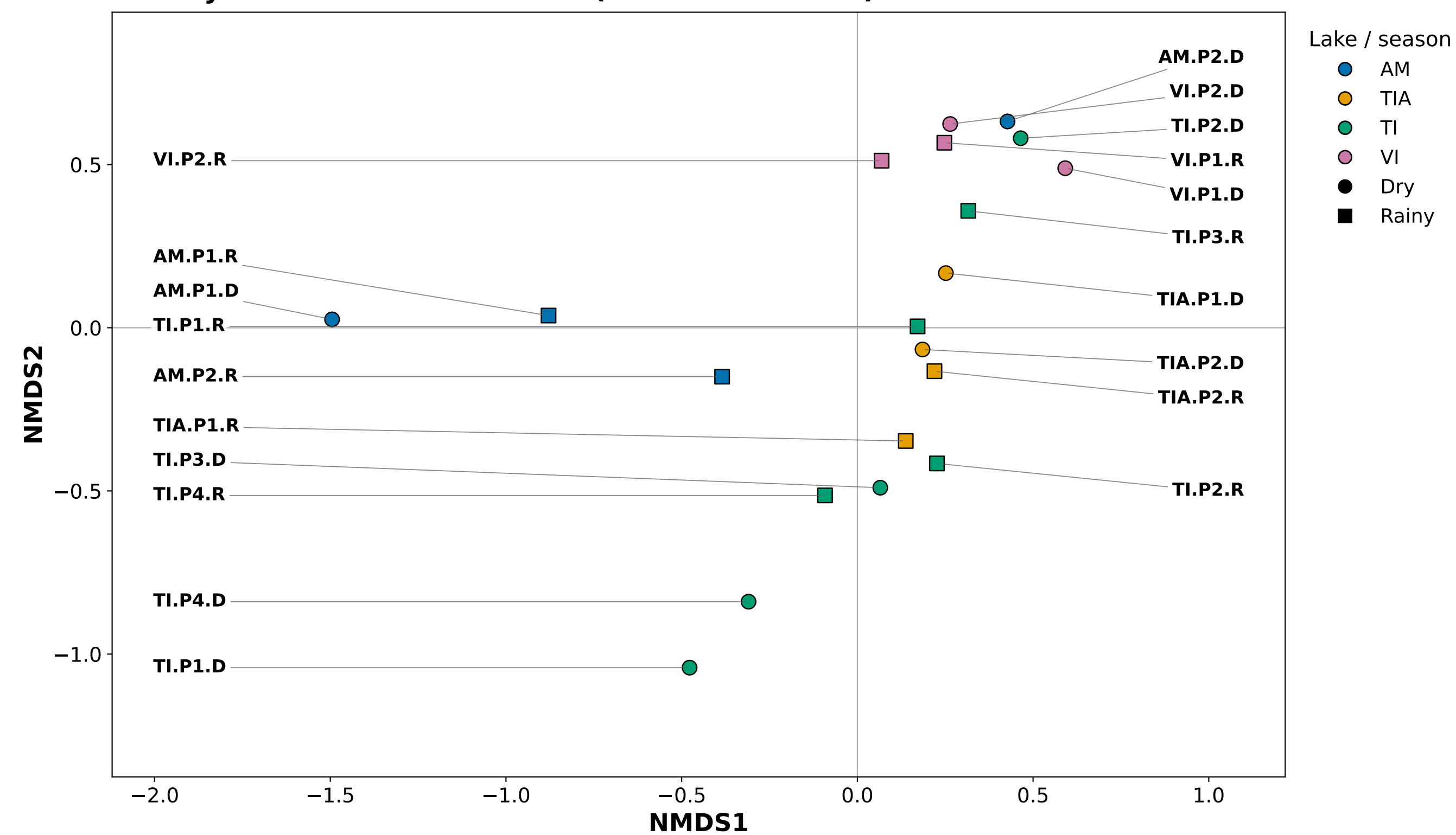
C Bray-Curtis non-metric MDS (Stress-1 = 0.065)
