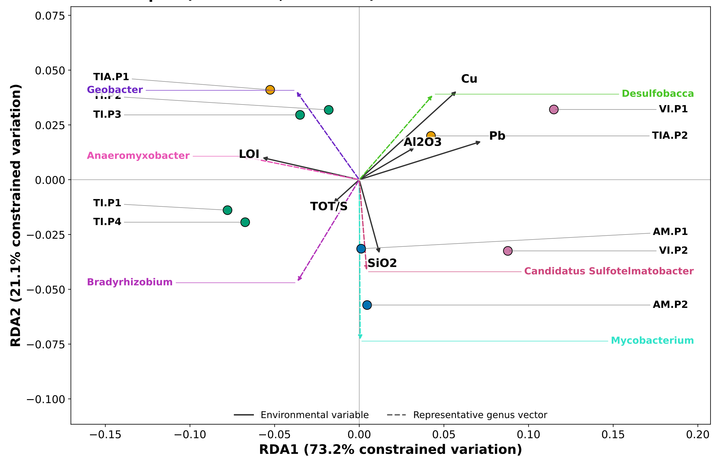
D RDA biplot ( R^2 = 0.671 ; P = 0.537 )
