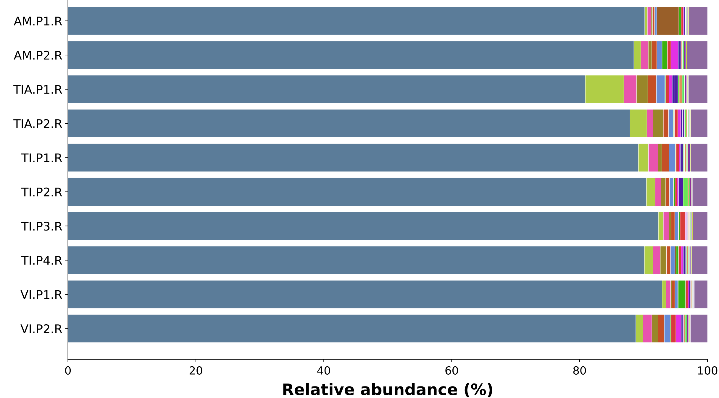
B Rainy-season genus profiles
