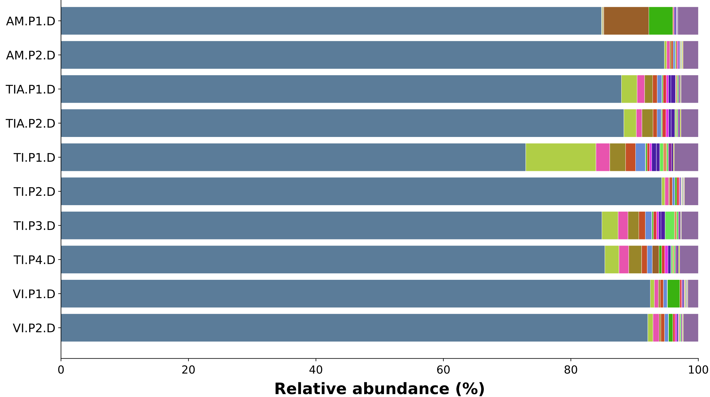
A Dry-season genus profiles
