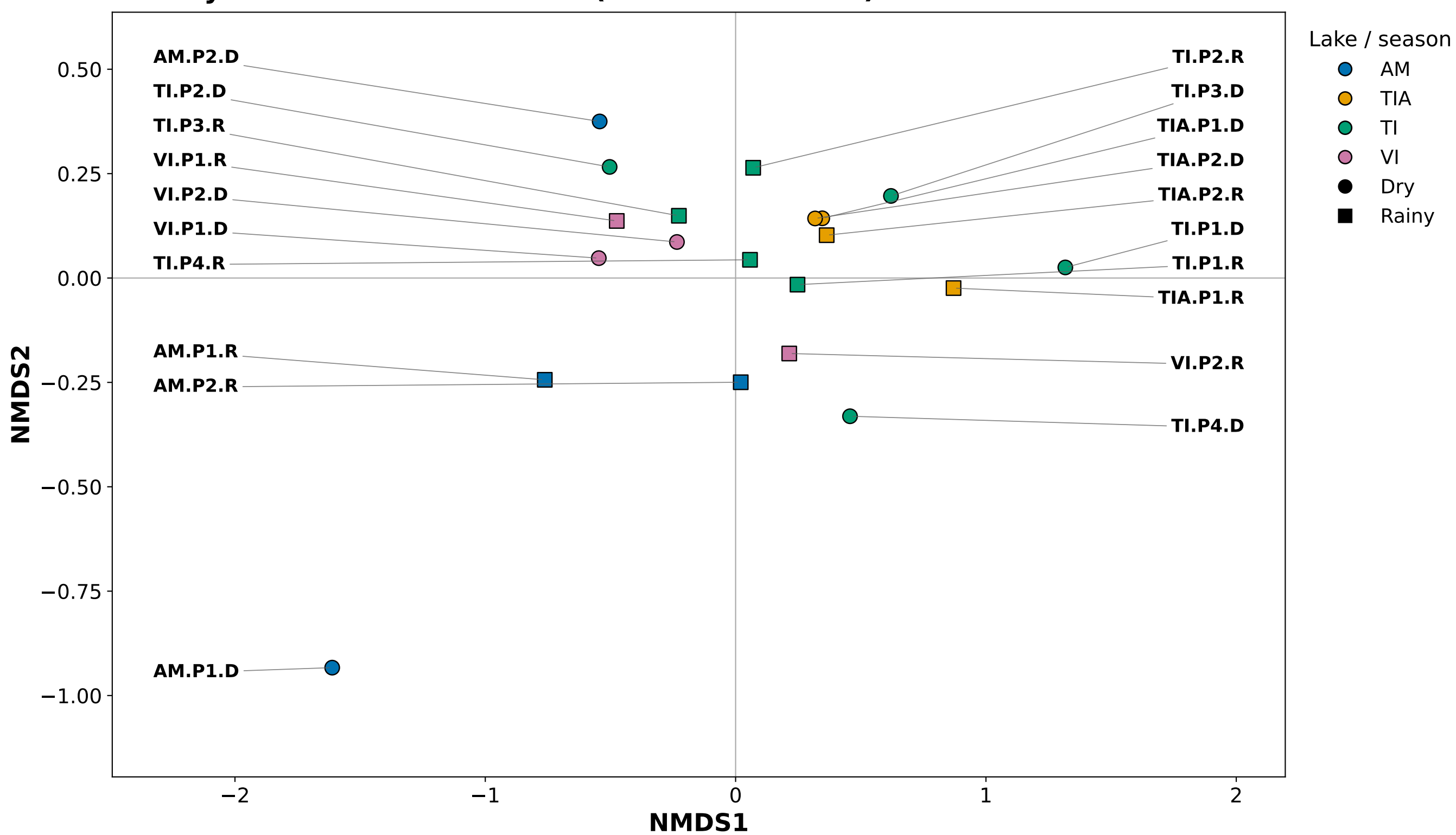
C Bray-Curtis non-metric MDS (Stress-1 = 0.054)
