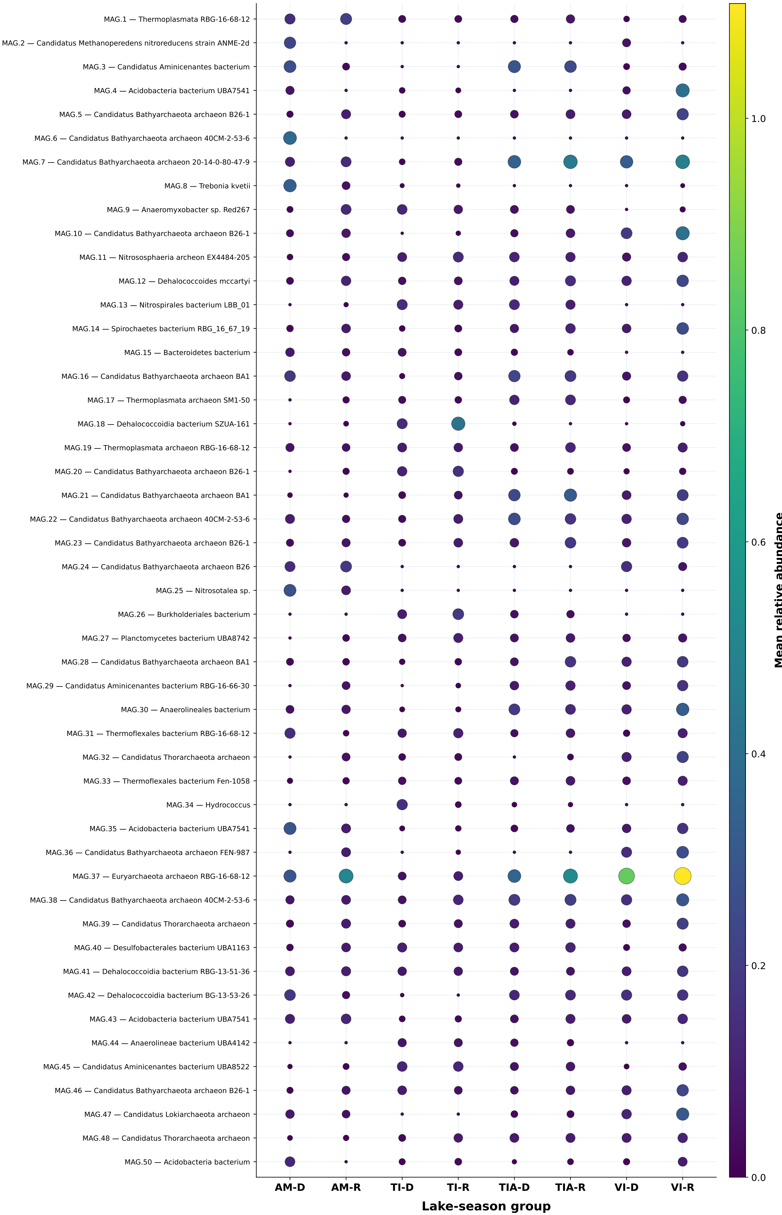
Relative abundance of all recovered metagenome-assembled genomes
