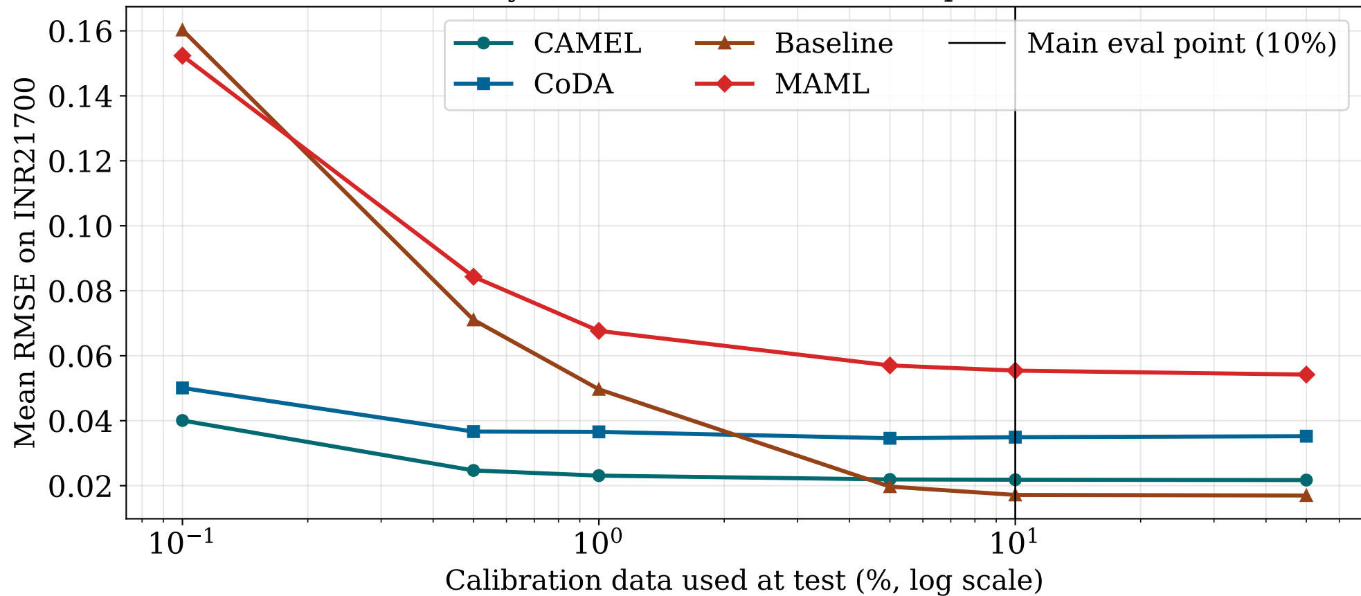
Sim-to-Real Data Efficiency on INR21700 (5 train-seed-paired evaluations, 20 tasks)
