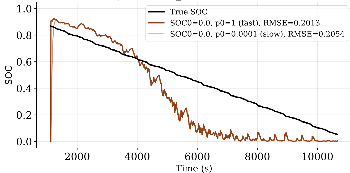
Baseline — recovery from SOC_0=0.0, p0 in {1, 0.0001}, calib=10%
