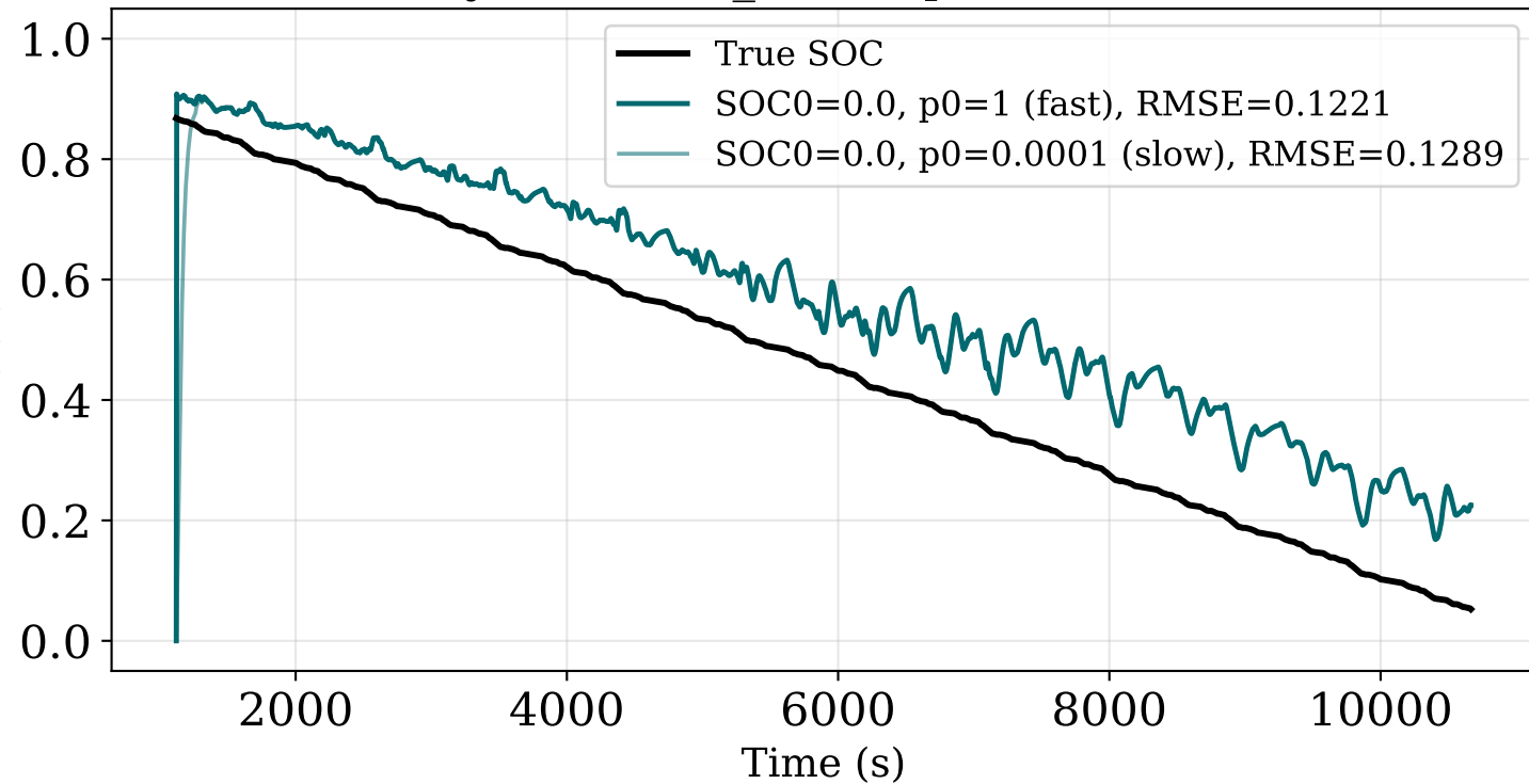
CAMEL — recovery from SOC_0=0.0, p0 in {1, 0.0001}, calib=10%
