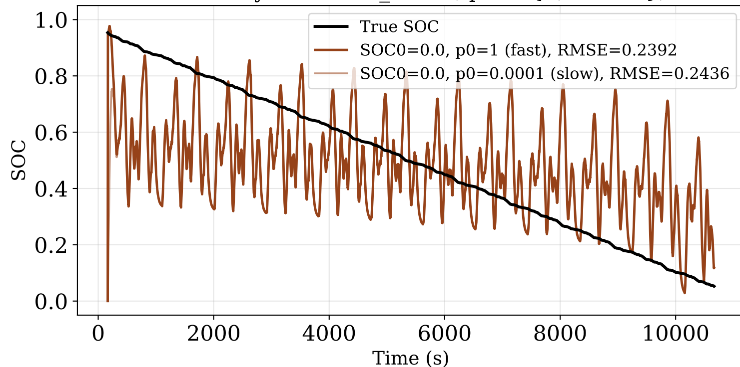
Baseline — recovery from SOC_0=0.0, p0 in {1, 0.0001}, calib=1%
