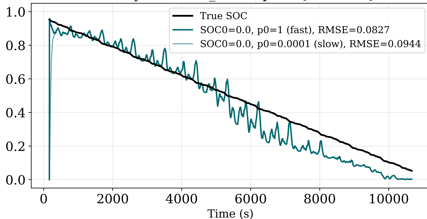
CAMEL — recovery from SOC_0=0.0, p0 in {1, 0.0001}, calib=1%
