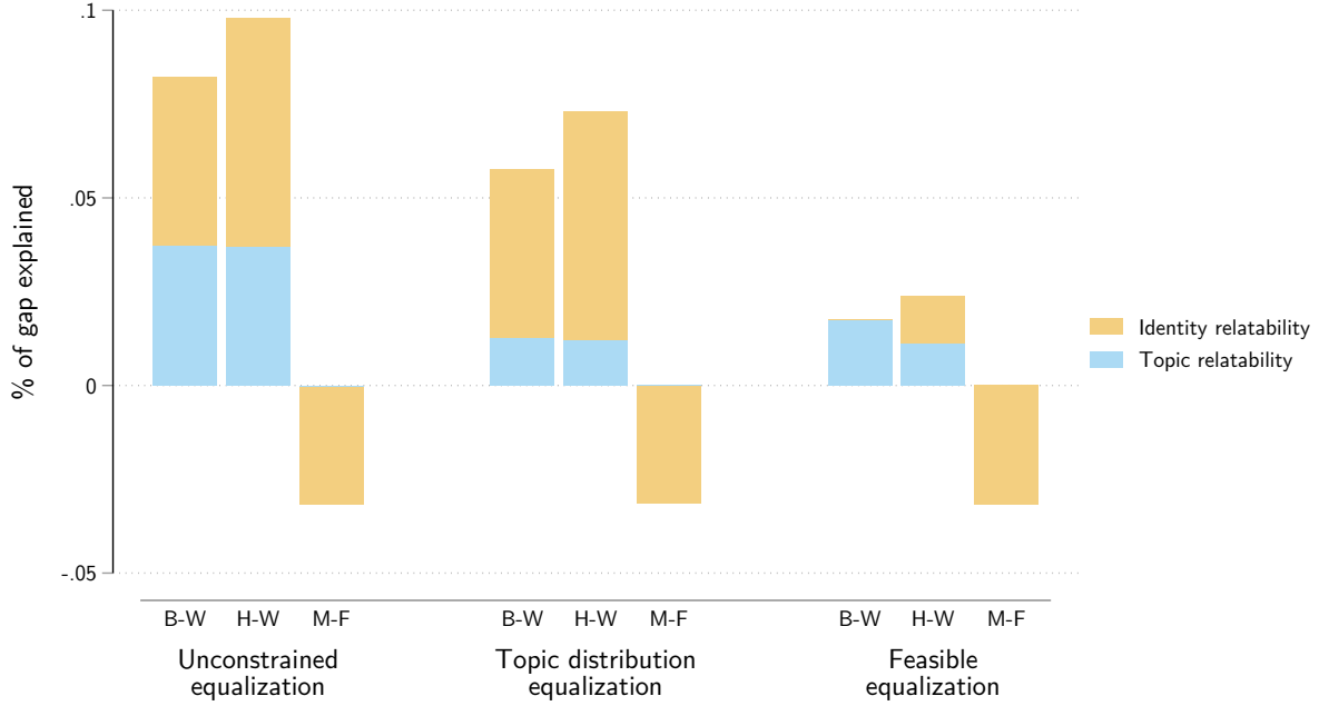
Figure 8: Estimated effect of equalizing relatability on demographic test score gaps
