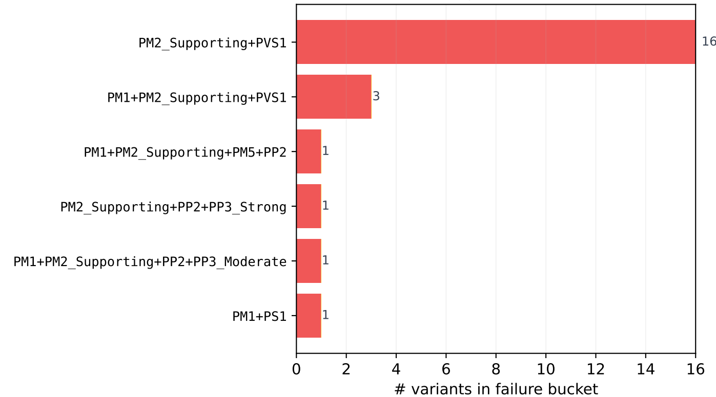
B truth (n=156,512; failed=23) top 8 criterion signatures of failed calls
