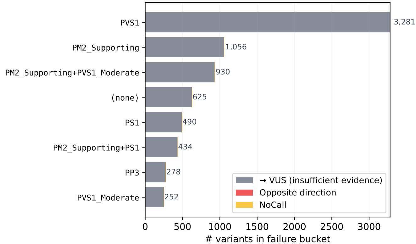
P truth (n=79,823; failed=8,636) top 8 criterion signatures of failed calls
