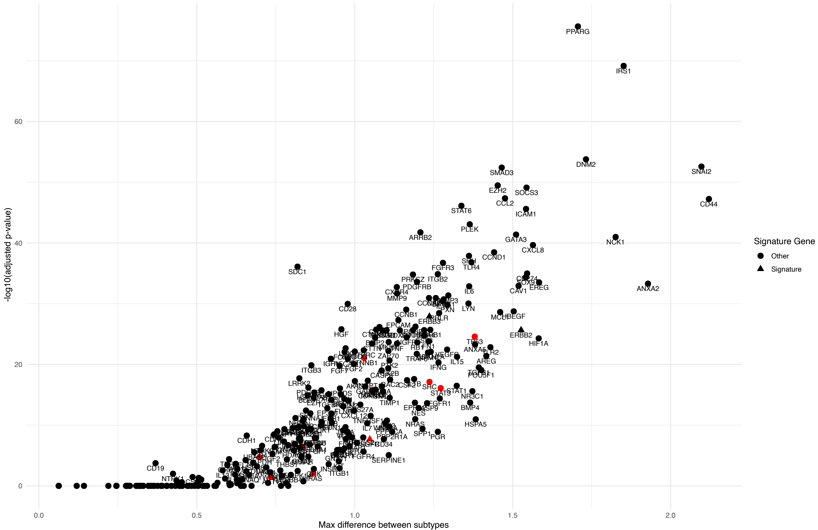
Volcano plot of ANOVA results
