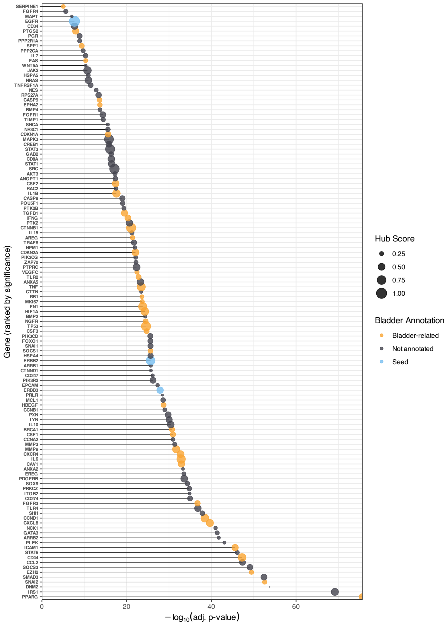
Lollipop Plot of Gene Significance
