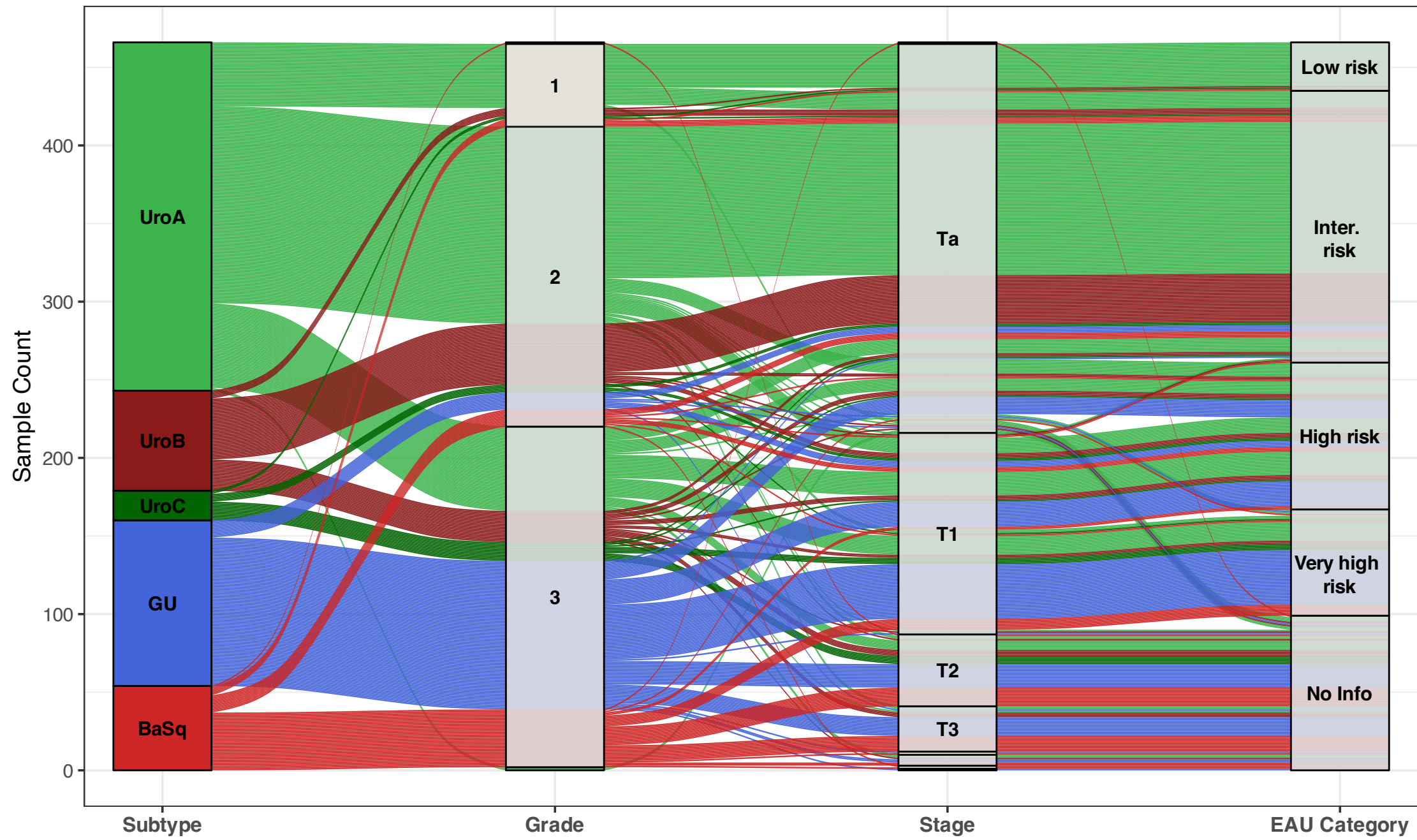
Sample Flow: Subtype → Grade → Stage → EAU Category
