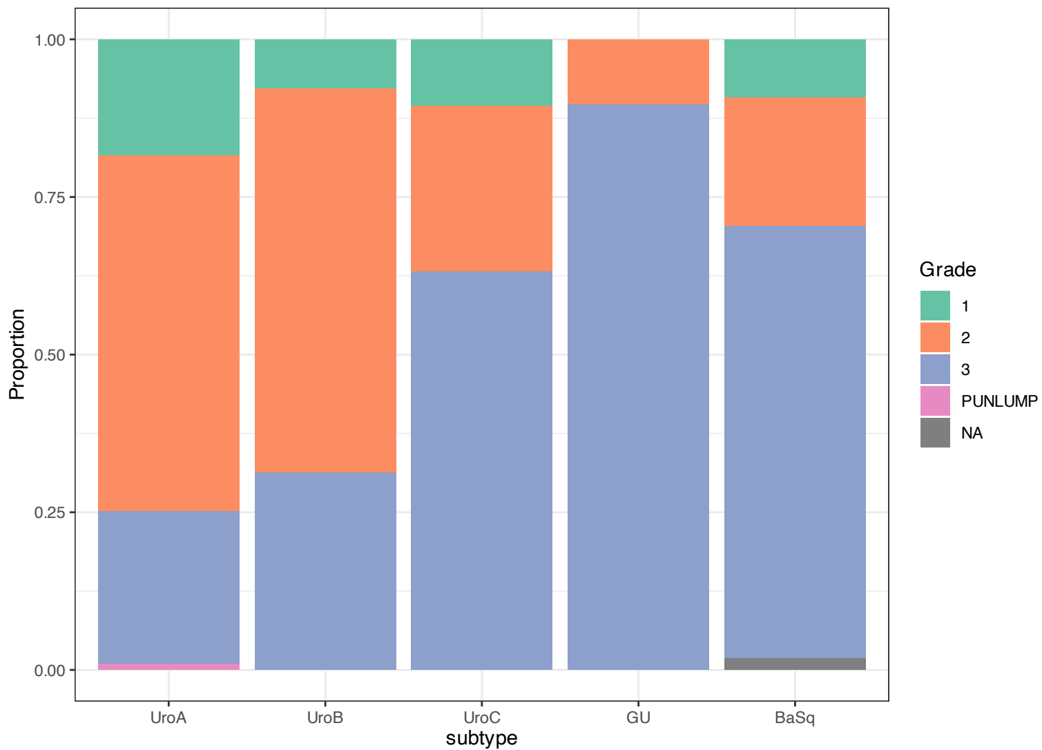
Grade Distribution within Subtypes
