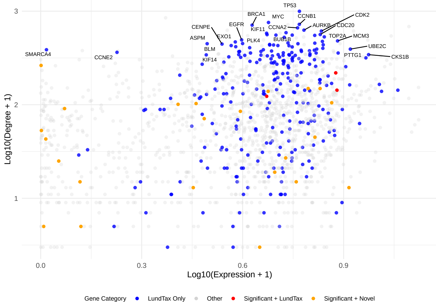
GU Subtype: Network Degree vs Expression
