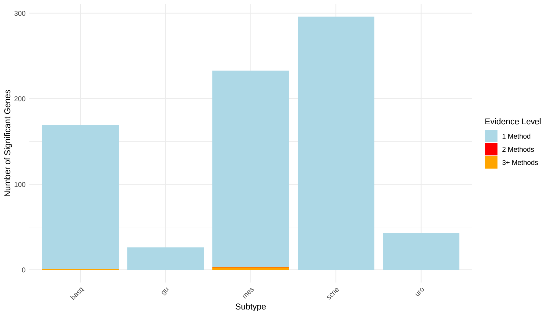
Number of Significant Genes by Evidence Level
