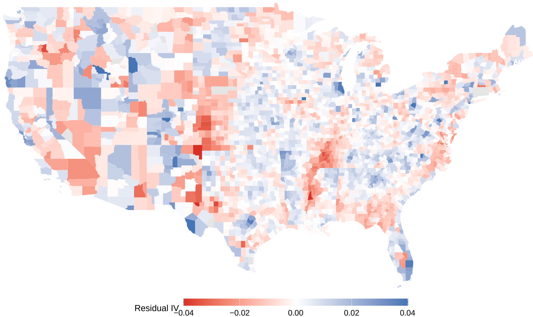
Panel B: Distance-Constrained Instrument ( \geq 500 km)
