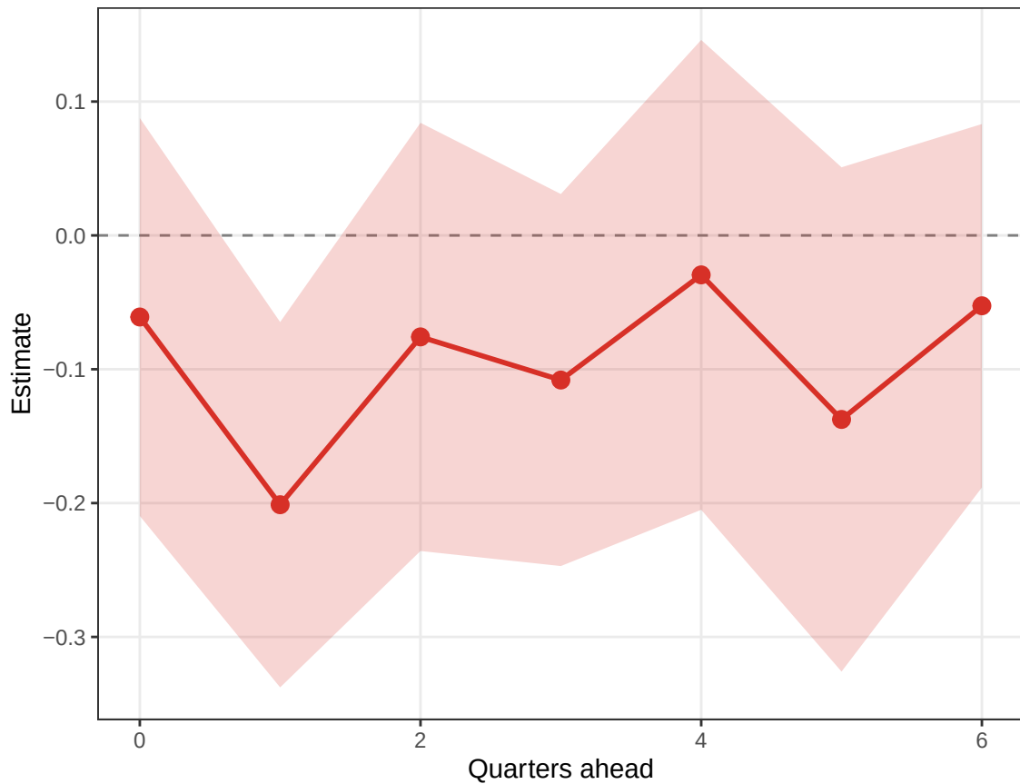
A. Incident \rightarrow Rules (h-period horizon)
