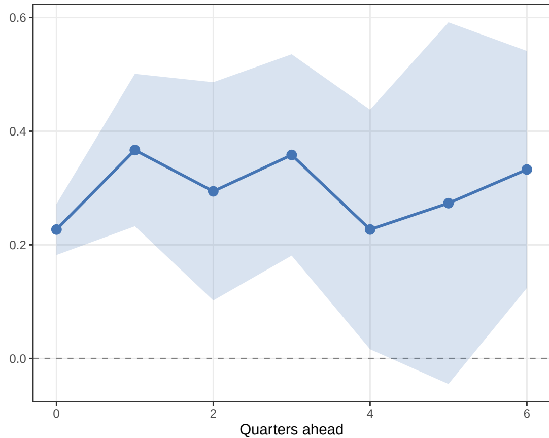
B. Burden \rightarrow Rules (persistent positive effect)
