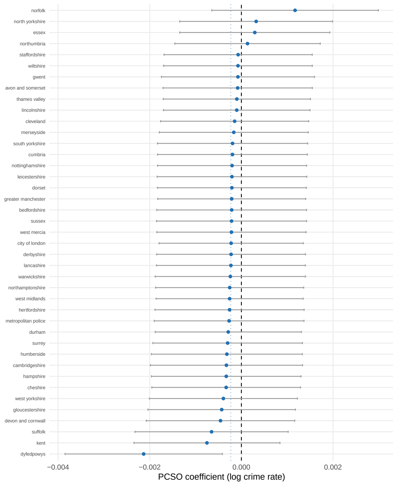
Figure 6: Leave-One-Out Jackknife
