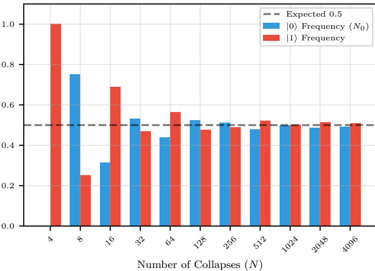
Quantum Superposition Measurement: H|0\rangle
