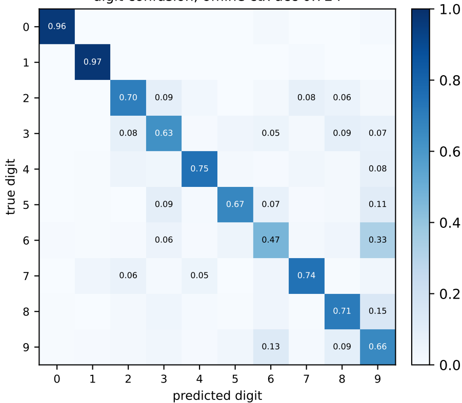
digit confusion, offline ctx acc 0.724
