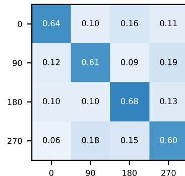
digit 9: 0.631
