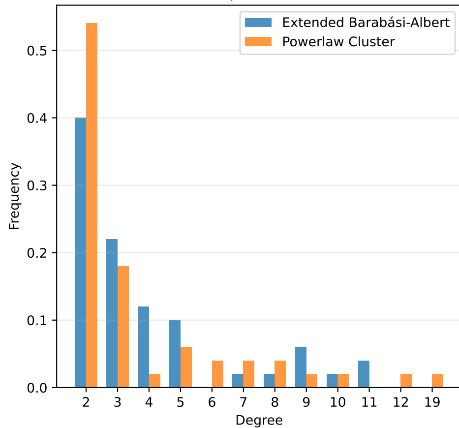
Graph Size: 50
