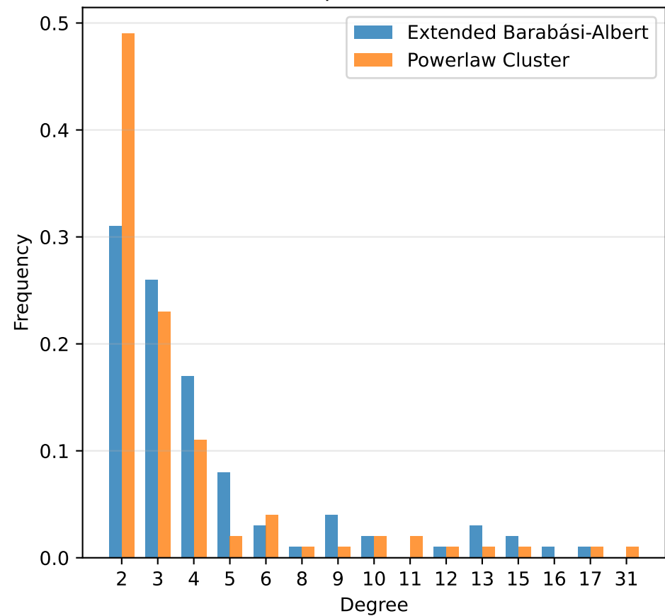
Graph Size: 100
