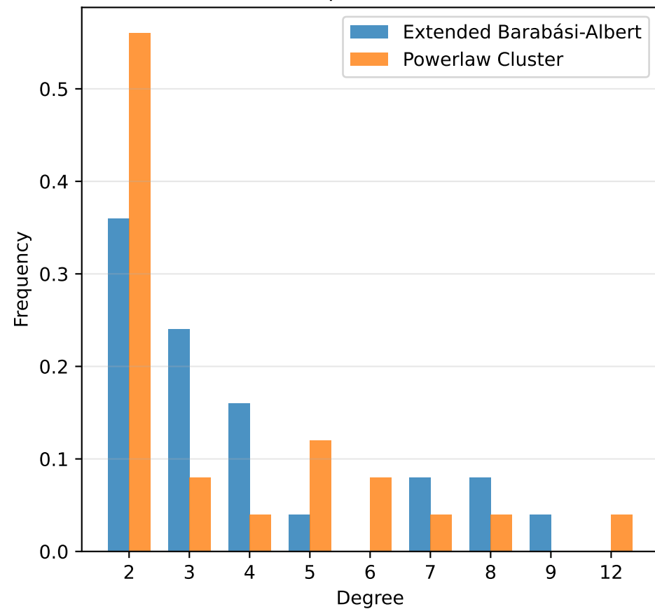
Graph Size: 25
