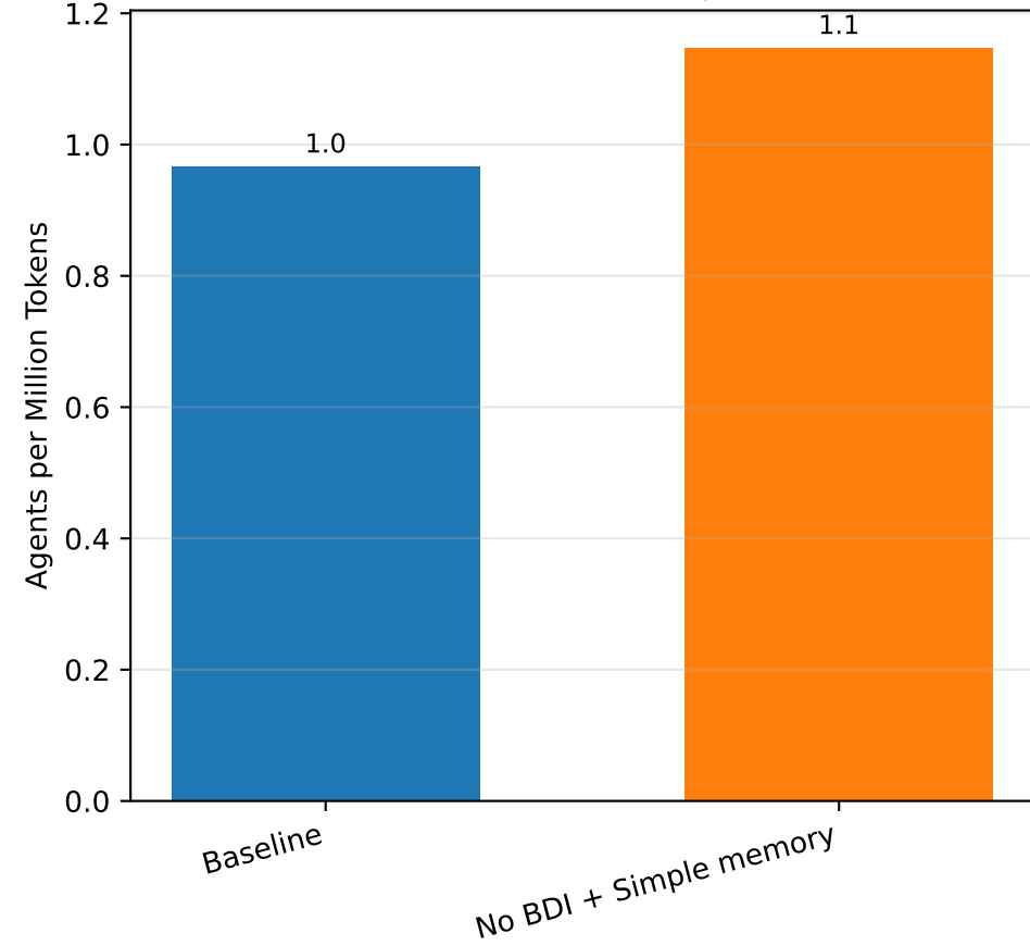
Token Efficiency
