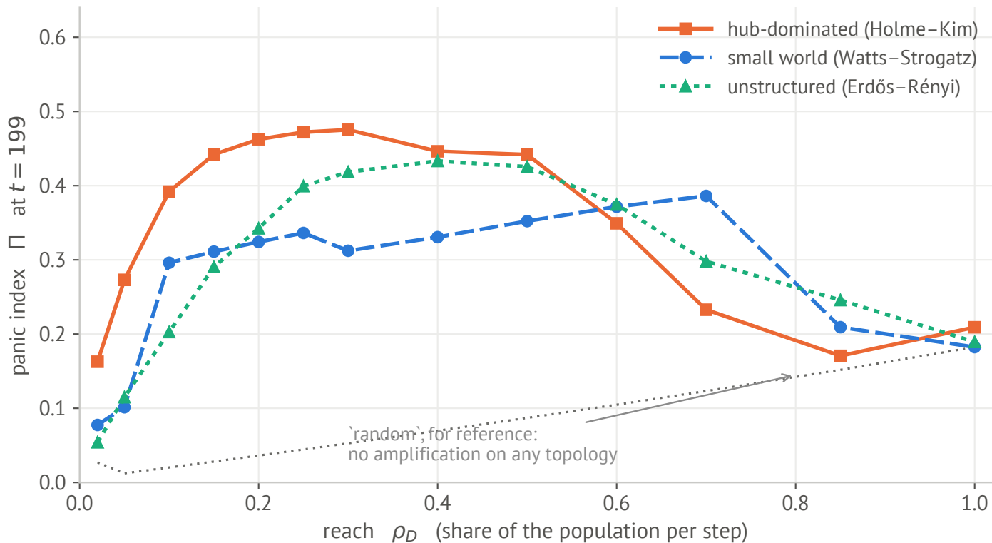
Panic index for the 'hub' repertoire across the three network generators
