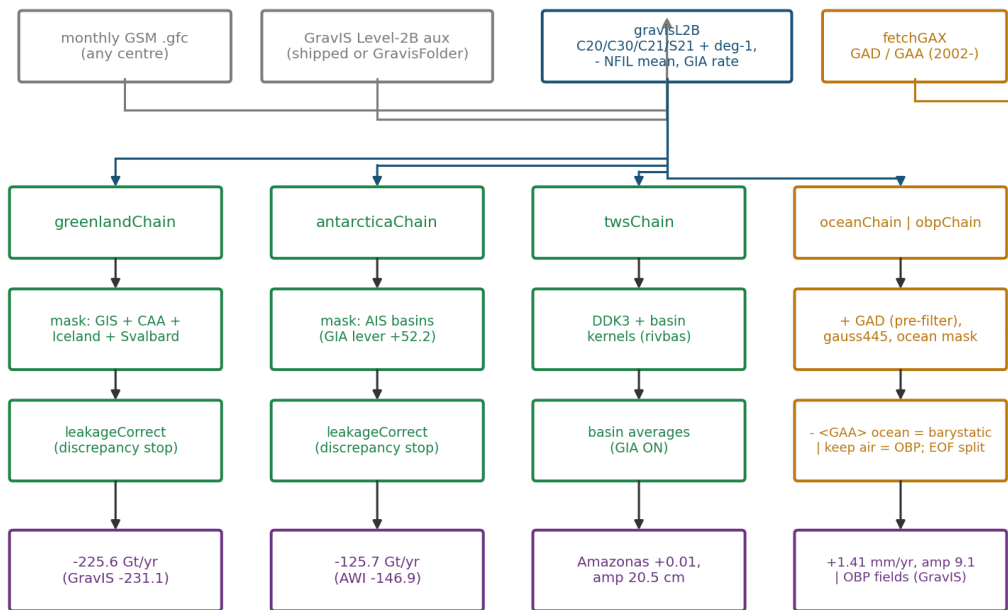
The chain family at v3.11.0: one shared gravisL2B core; the ocean lane forks after GAD into barystatic ( oceanChain , with EOF circulation split) and bottom pressure ( obpChain ).
