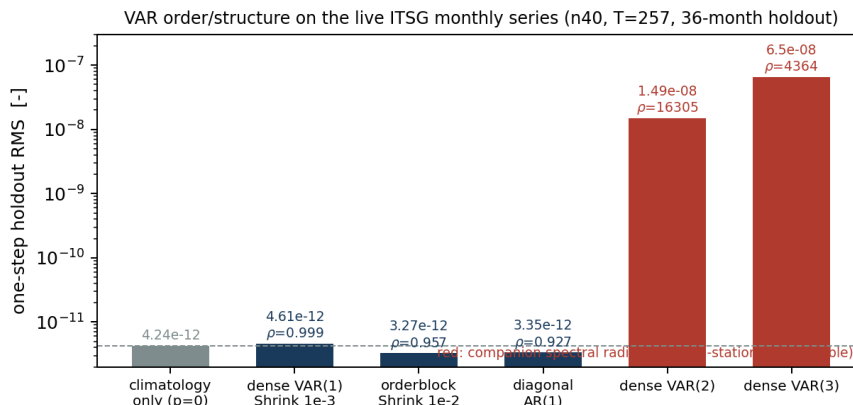
Figure: one-step holdout RMS per process model on the live monthly series. The dense VAR(1) at weak shrink is WORSE than no dynamics at all (overfit at T \approx 0.13 P ); the structured estimators beat climatology-only by 21–23%; p \geq 2 explodes. Order = 1 confirmed.
