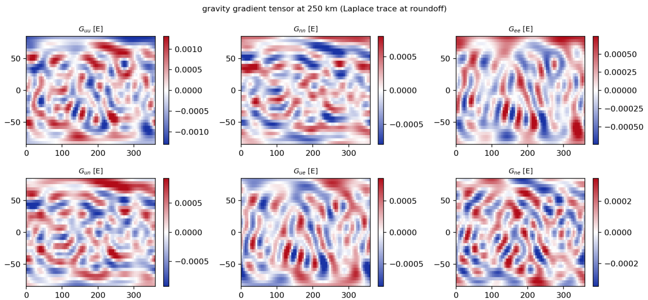
D11 — All six gradient tensor components at 250 km in Eotvos. The Laplace invariant G_{nn} + G_{ee} + G_{uu} = 0 holds at roundoff (4e-15 of max|G| here) — a full-chain check of first and second Legendre derivatives, trig derivatives and frame terms at once.
