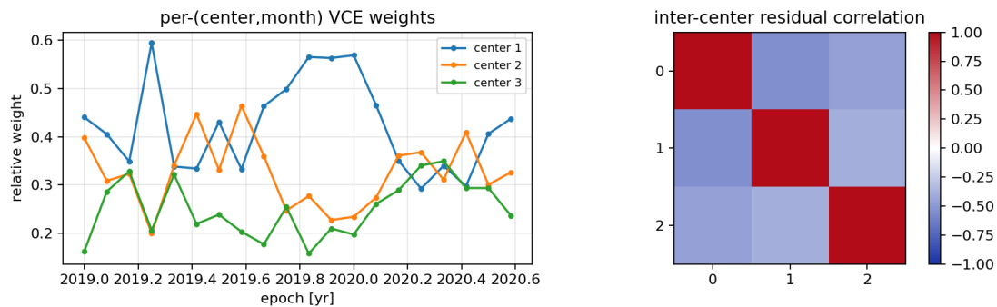
D14 — Multi-center VCE: per-(center, month) weights track the time-varying noise levels; the inter-center residual correlation matrix is the honesty diagnostic — VCE assumes independence, GRACE centers share data and background models.
