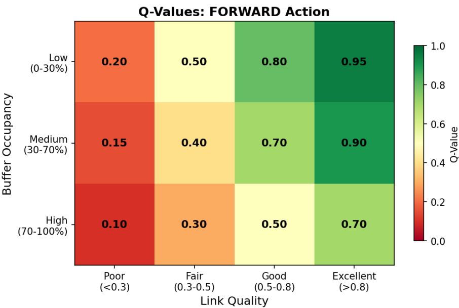
AETHERIX RL Routing Agent: Decision Heatmaps
