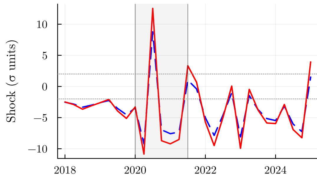
Investment ( \varepsilon_{qs} )
