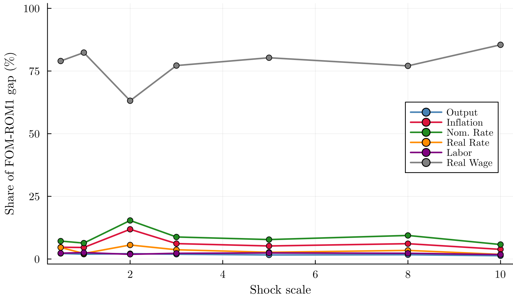
Gali (no ZLB): observable-block decomposition
