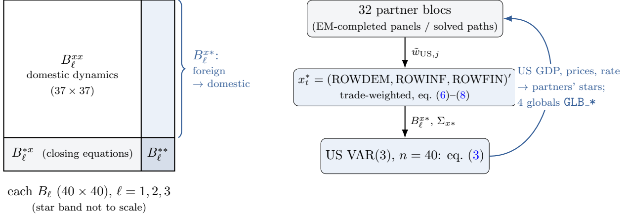
Figure 1: Left : where the foreign variables enter — the shaded column block B_\ell^{x*} gives each of the 37 domestic equations its nine foreign regressors; the bottom rows are the stars’ own (closing) equations. Right : the two-way linkage. The US is both a receiver (its stars aggregate its partners) and the source of the four global commons; the feedback loop is closed at estimation time by the EM star iteration and at solve time by the fixed point of Section 7.
