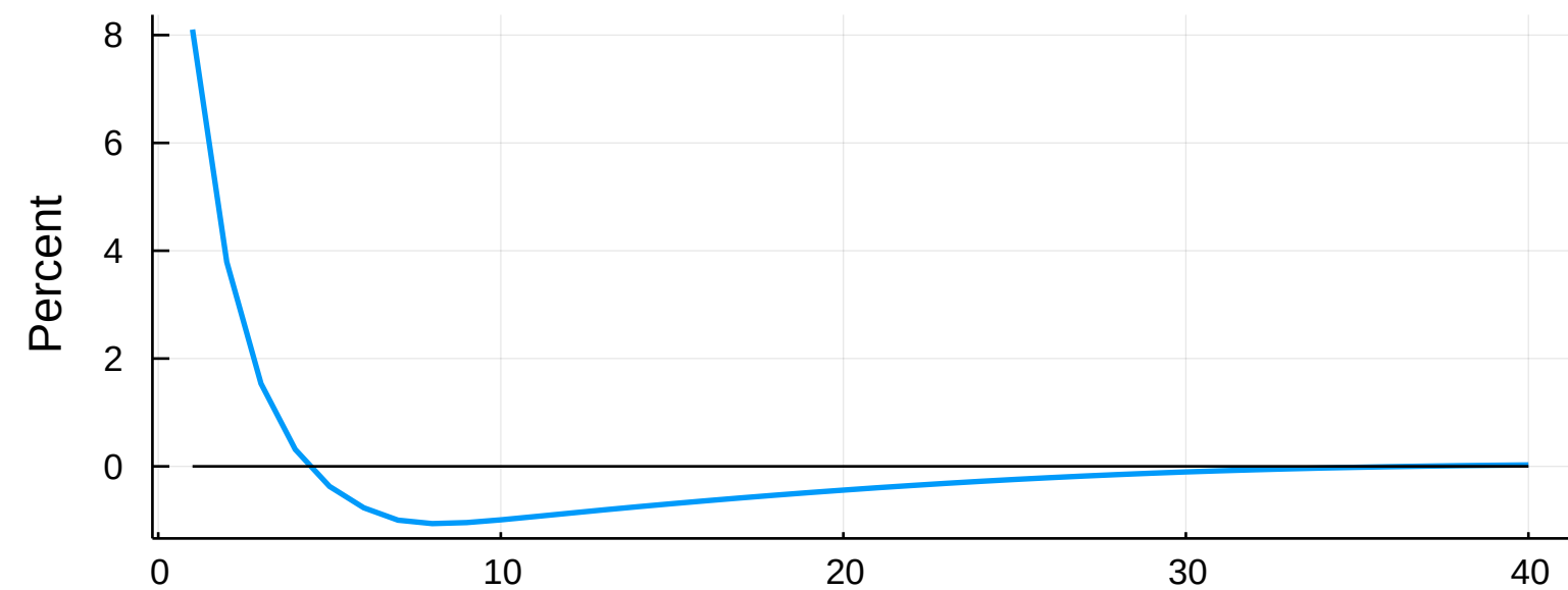
Ex- ante real rate
