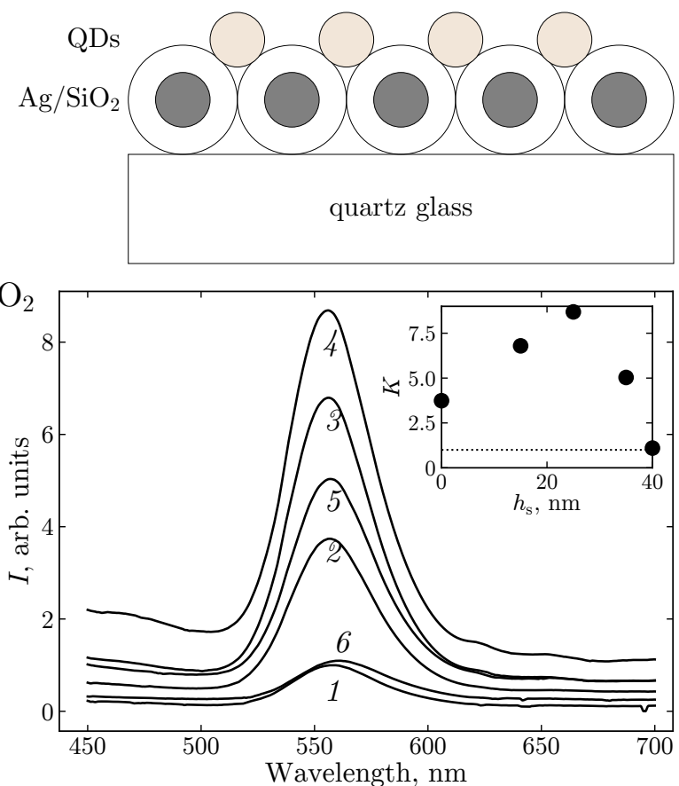
Figure 8. Schematic of the structures for studying plasmonic enhancement, and PL spectra of \text{CdSe/ZnS} QDs without (1) and near plasmonic particles with a shell thickness h_s = 0 (no shell) (2), 15 (3), 25 (4), 35 (5), and 40 nm (6). Inset: enhancement factor versus shell thickness
