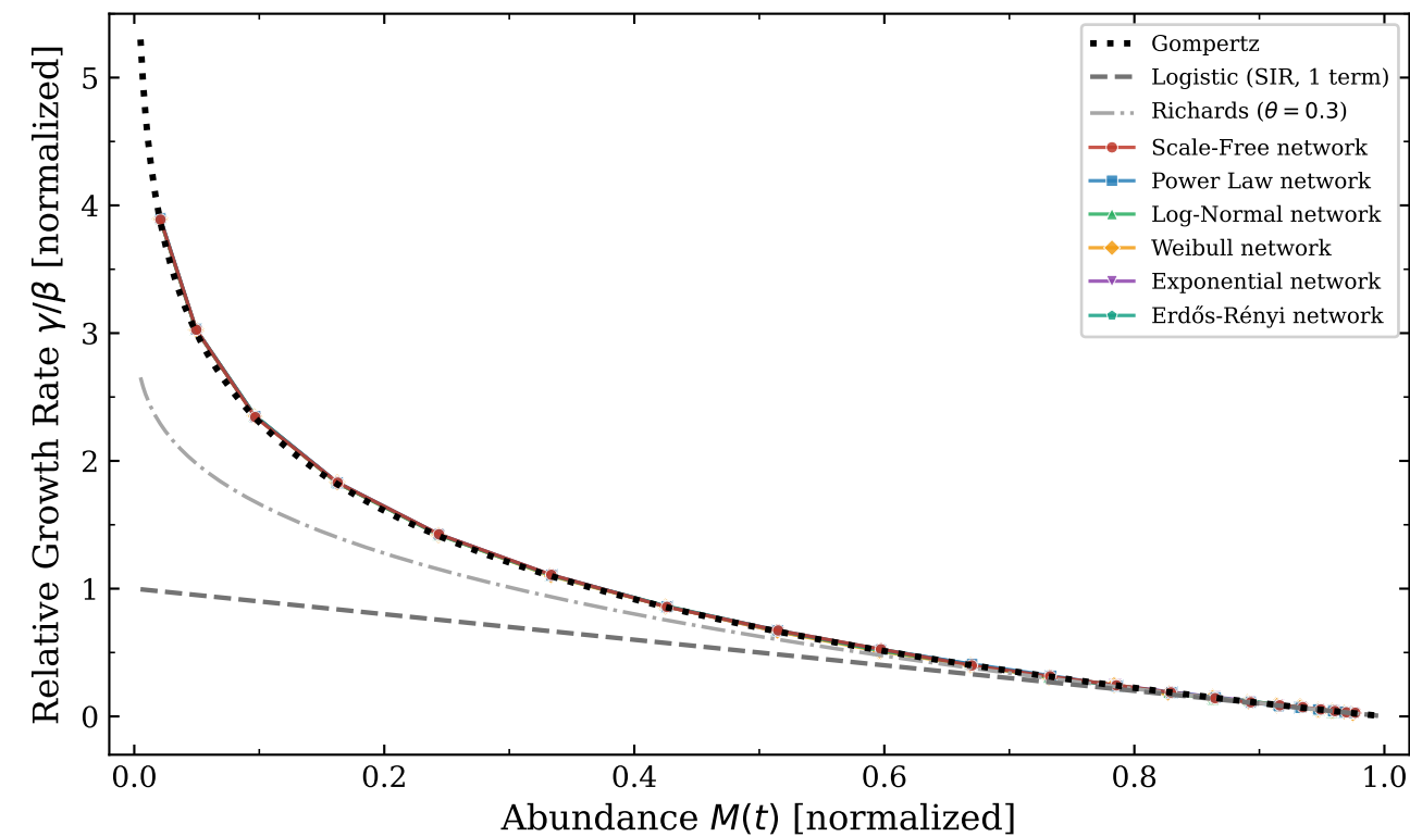
(a) Relative growth rate
