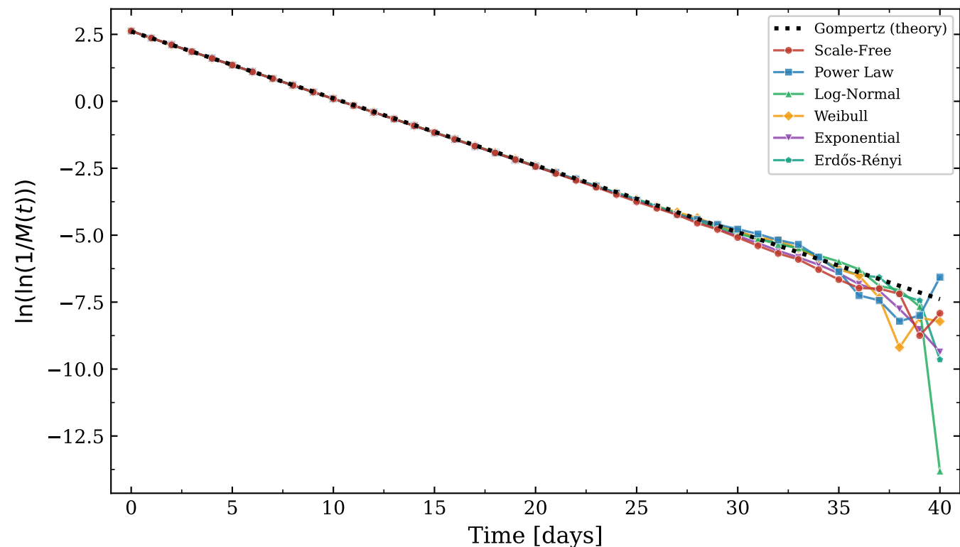
(b) Double-log transform
