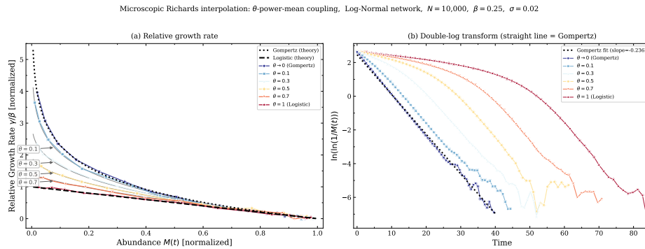
Figure 2: Different simulated Richard growth models are compared with their theoretical curves, using a Log-Normal network with 10,000 nodes and mean-field approximation. Note that the higher values of \theta makes the growth unstable as discussed in the text.
