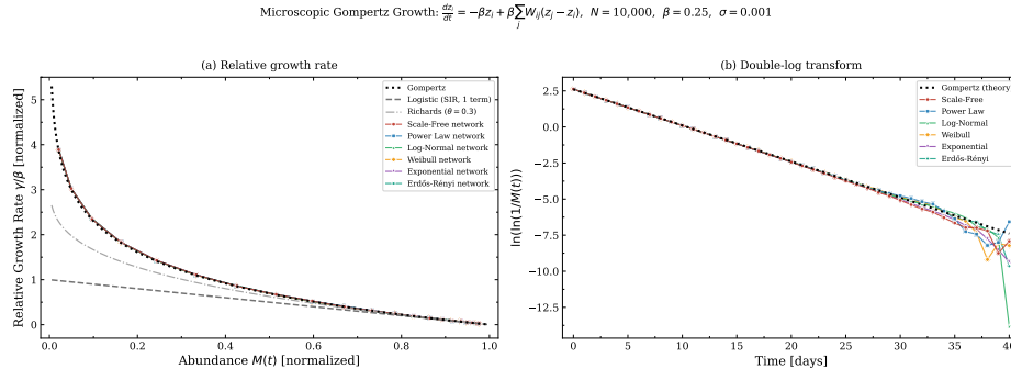
Figure 3: Comparison of relative growth rates for different networks under a microscopic Gompertz mode with 10,000 nodes using a mean field approximation, showing fidelity to the theoretical limit regardless of the underlying network. Different networks plotted in color, showing minimal deviation from the theoretical gompertz curve. A logistic and Richards \theta = 0.3 theoretical curve is plotted for comparison. The abundance variable is normalized to values between 0 and 1.
