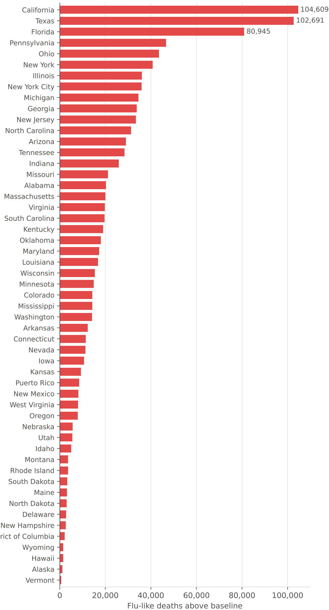
Excess flu-like deaths, 2020-2021
