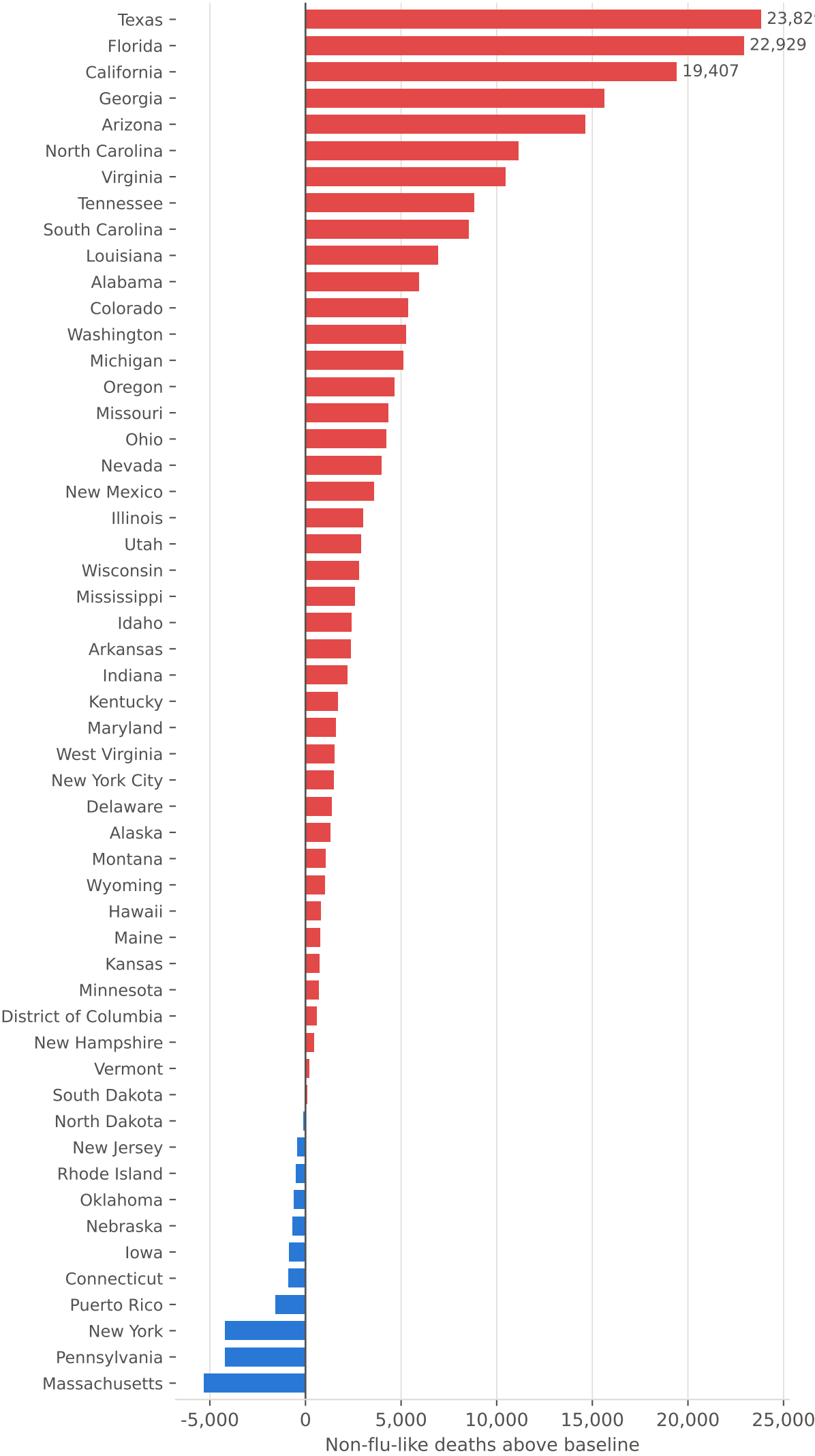
Excess non-flu-like deaths, 2020-2021
