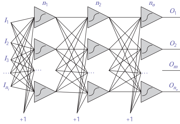
FIGURE 12.3 Three-layer multilayer perceptron network: the number of inputs is n_i , the number of outputs is n_o , and n_1 and n_2 are the numbers of neurons in the first and second layers separately.
