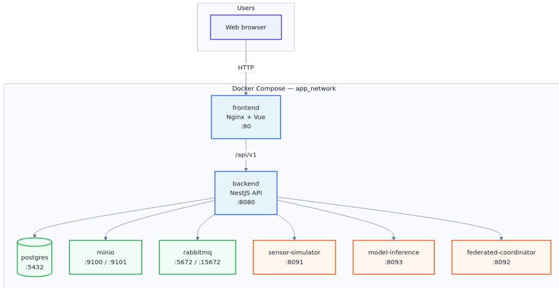
Figure 4.3: Docker Compose deployment topology.
